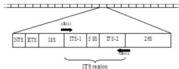
Figure 1. Organization of ITS region of nrDNA with location of primers used in this study. Information of primers is also provided.
