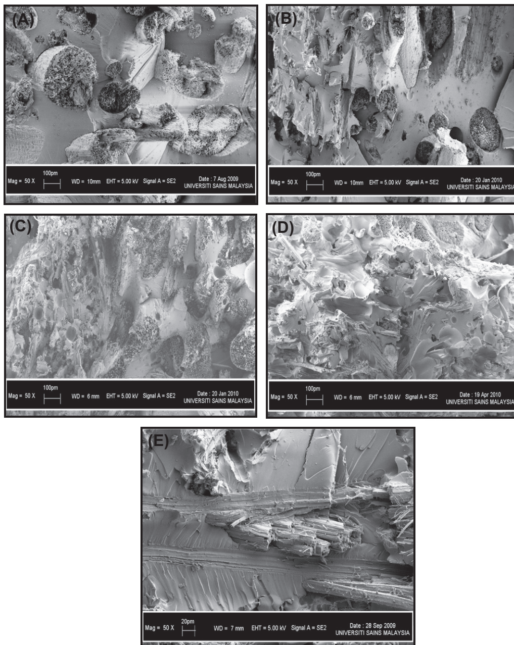
Fig. 1. SEM micrographs of tensile fracture of (A) EFB composite, (B) oil palm EFB:jute (4:1) hybrid composite, (C) oil palm EFB:jute (1:1) hybrid composite, (D) oil palm EFB:jute (1:4) hybrid composite, and (E) jute composite.
