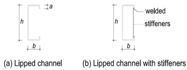
Figure 2. Vertically stiffener
